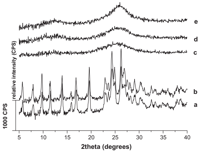
Fig. 4. XRD diffractograms of (a) sodium cromoglicate raw material (Sigma) (b) micronised sodium cromoglicate (Intal®), (c) spherical NPMPs of sodium cromoglicate (spray dried from water:methanol:n-butyl acetate (v/v) 1:15:15), (d) non-spherical NPMPs of sodium cromoglicate (spray dried from methanol:n-butyl acetate (v/v) 95:5) and (e) non-porous spray dried sodium cromoglicate (spray dried from water).
