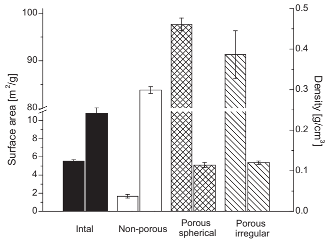
Fig. 6. Surface area and bulk density measurements of micronised sodium cromoglicate, non-porous spray dried sodium cromoglicate, spherical NPMPs of sodium cromoglicate (spray dried from water:methanol:n-butyl acetate (v/v) 1:15:15) and non-spherical NPMPs of sodium cromoglicate (spray dried from methanol:n-butyl acetate (v/v) 95:5). The left bar refers to surface area (mean ± sd, n = 4) and the right bar refers to bulk density (mean ± sd, n = 3).
