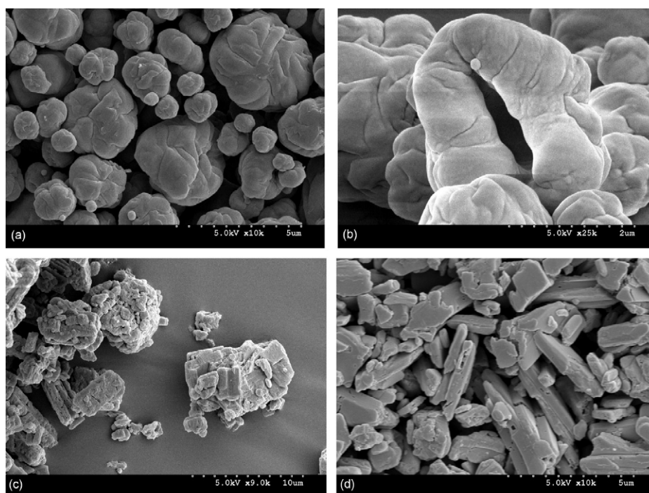
Fig. 1. SE micrographs of (a and b) spray dried non-porous sodium cromoglicate from an aqueous solution, (c) sodium cromoglicate raw material (Sigma sample) and (d) micronised sodium cromoglicate (Intal® Spincaps). Note different magnifications.
