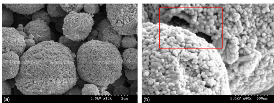
Fig. 3. SE micrographs of spray dried sodium cromoglicate from different cosolvent systems of water:methanol:n-butyl acetate 1:15:15 (v/v). Note the different magnification of SEM micrographs.
